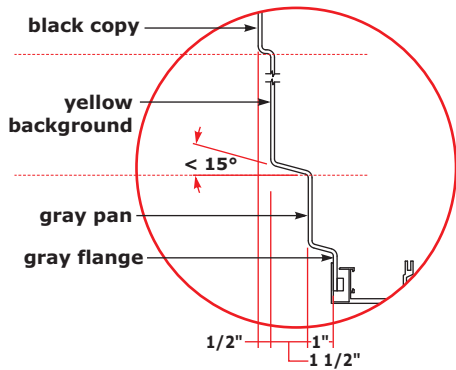
FACE EMBOSMENT DETAIL
