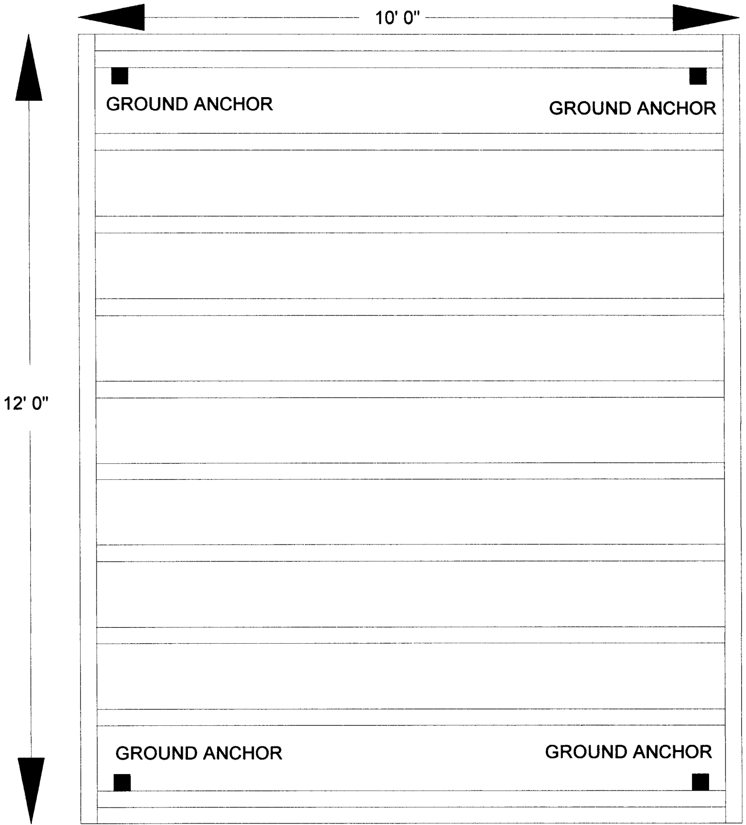
JOIST LAYOUT WITH GROUND ANCHORS
