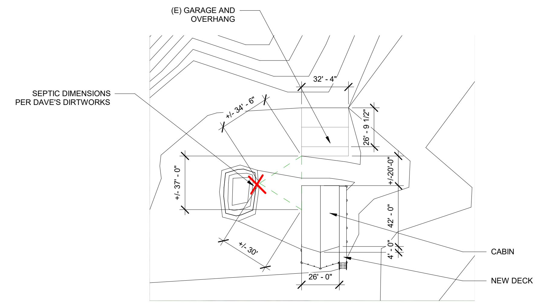
② SITE PLAN - Callout 1 1" = 40'-0"
