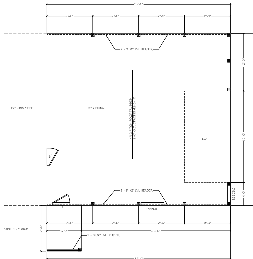
FLOOR PLAN
