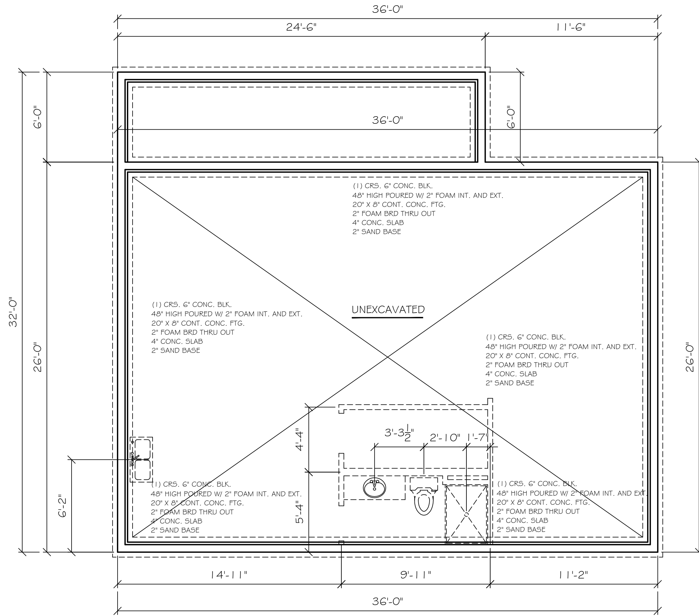
FOUNDATION PLAN 1/4" = 1'-0"
